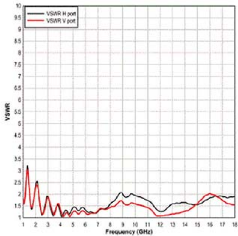
Model 3164-11 Open Boundary Quad-Ridged Horn VSWR
