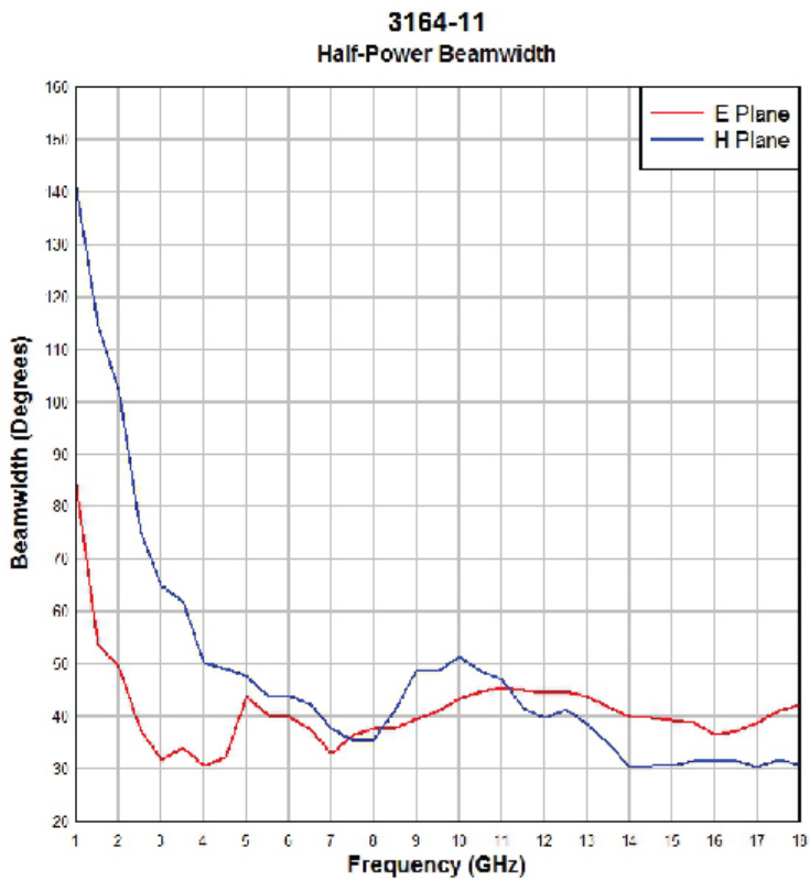
Model 3164-11 Open Boundary Quad-Ridged Horn Half-Power Beamwidth
