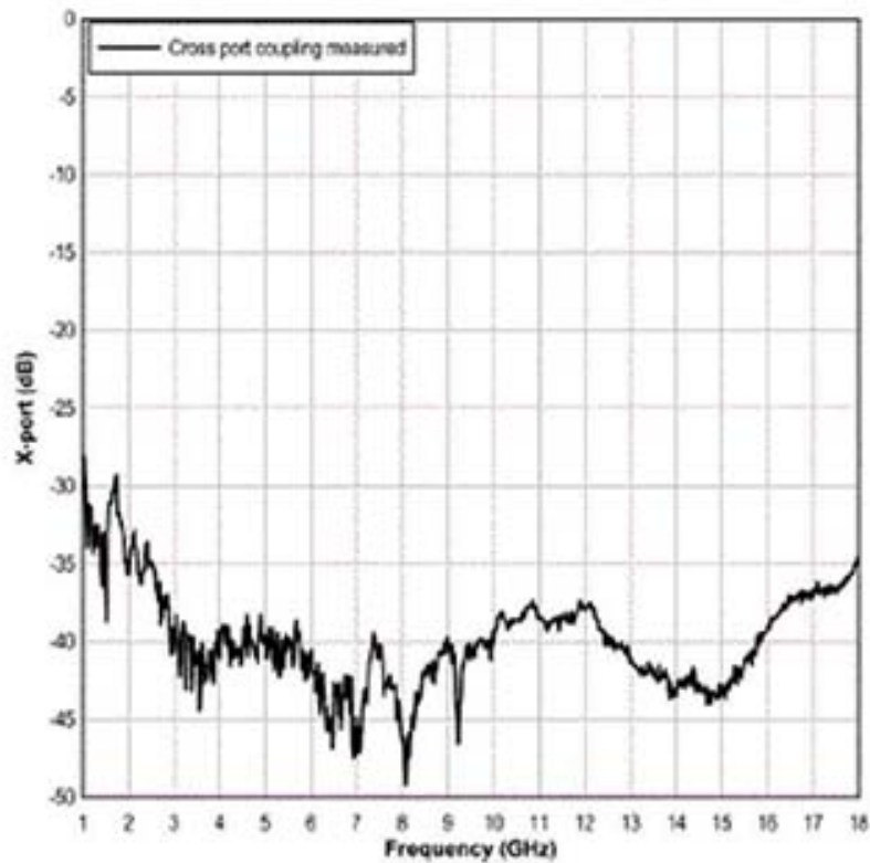
Model 3164-11 Open Boundary Quad-Ridged Horn Typical Radiation Patterns Cross Port Coupling
