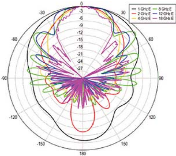
Model 3164-11 Open Boundary Quad-Ridged Horn Typical Radiation Patterns E Plane
