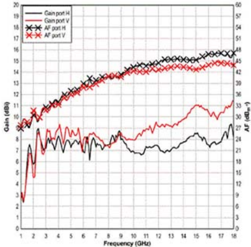
Model 3164-11 Open Boundary Quad-Ridged Horn Antenna Factors and Gain
