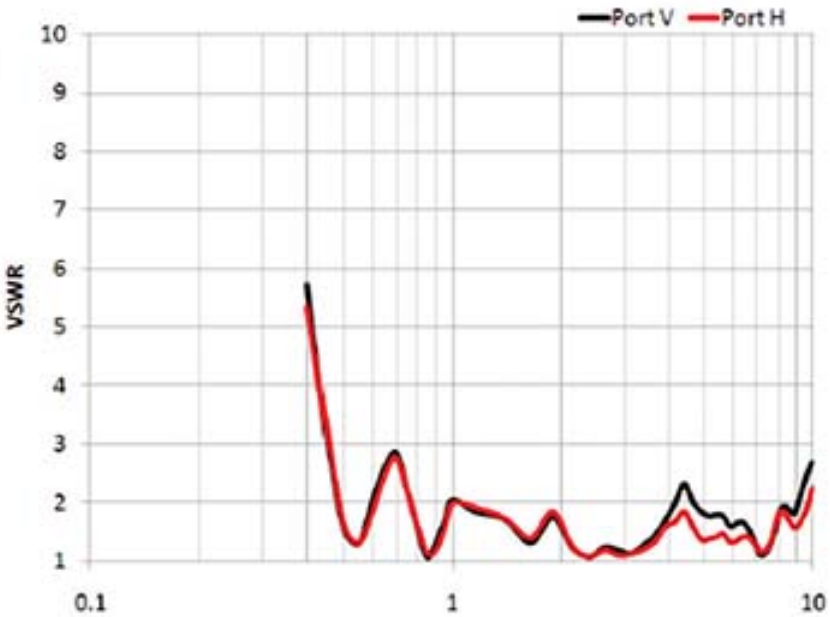
Model 3164-10 Open Boundary Quad-Ridged Horn VSWR
