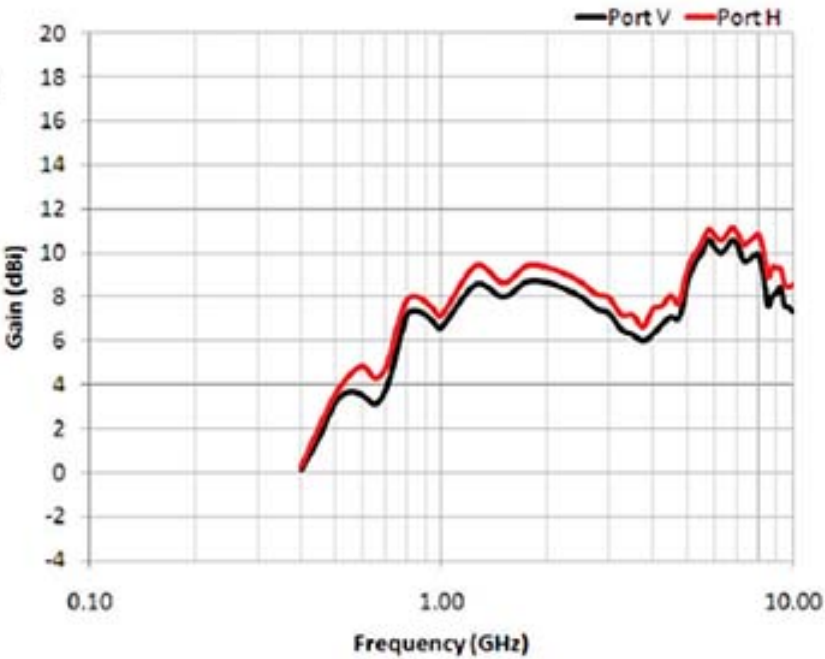
Model 3164-10 Open Boundary Quad-Ridged Horn Gain
