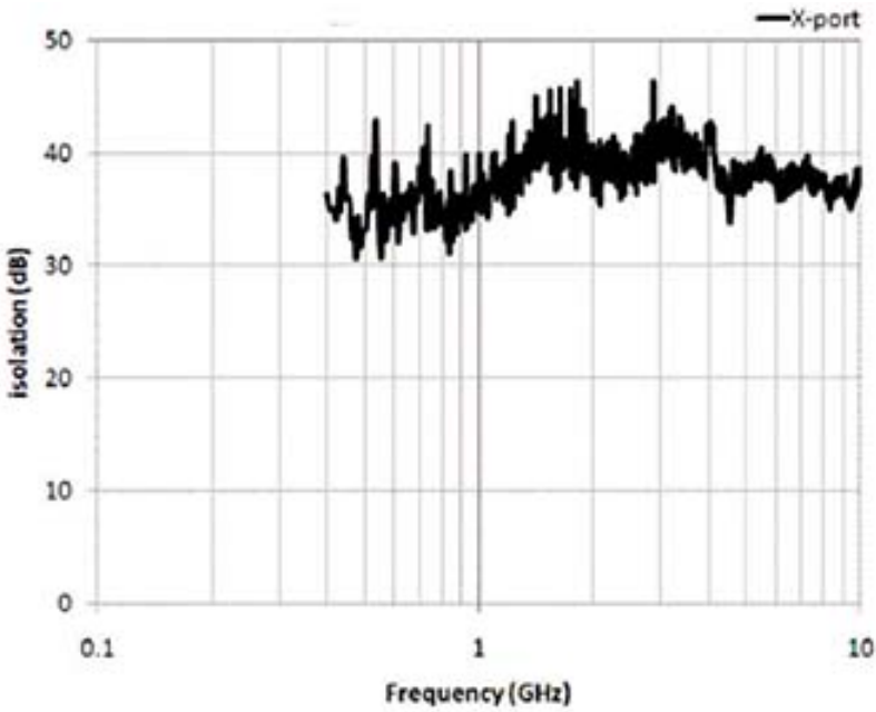
Model 3164-10 Open Boundary Quad-Ridged Horn Cross Port Isolation
