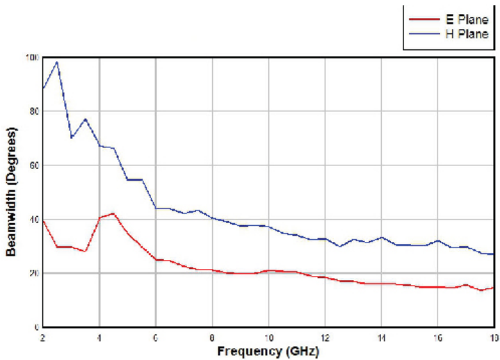
Model 3164-05 Open Boundary Quad-Ridged Horn Half-Power Beamwidth
