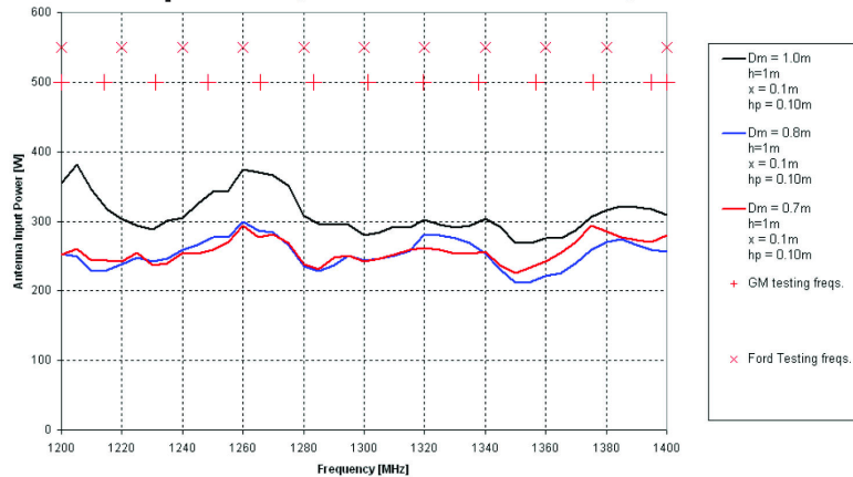
Antenna Input Power, Horizontal Polarization, With Test Points
