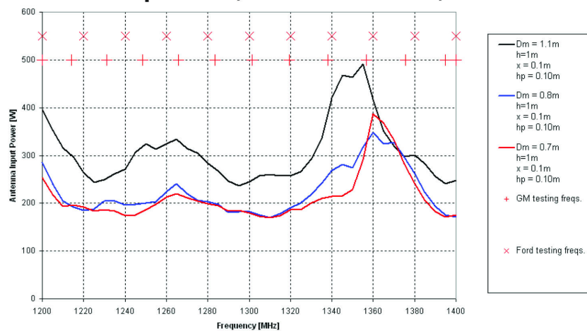
Antenna Input Power, Vertical Polarization, With Test Points
