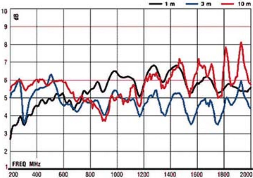
3148B Log Periodic Dipole Array Antenna Gain
