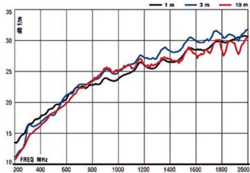
3148B Log Periodic Dipole Array Antenna Factor
