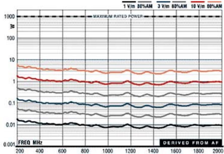
3148B Log Periodic Dipole Array Antenna Forward Power at 1 m
