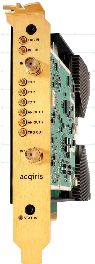
Figure 10. Open view of the SA220P.
