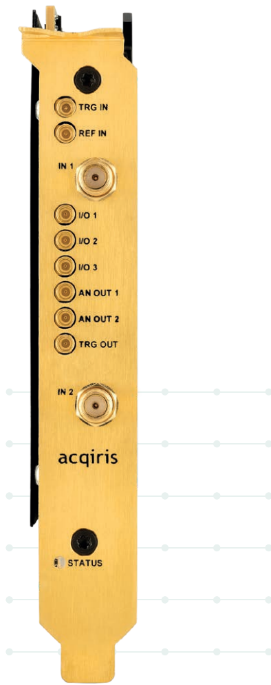
Figure 3. SA220P front panel, with analog inputs and multiple programmable I/O signals.
