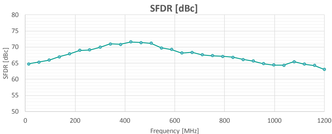
Figure 9. The SA220E offers stable signal performance across the overall bandwidth. Above figure corresponds to the SNR and SFDR measured on 16 channels, at 25°C, 0.5 V FSR, -1 dBFS.
